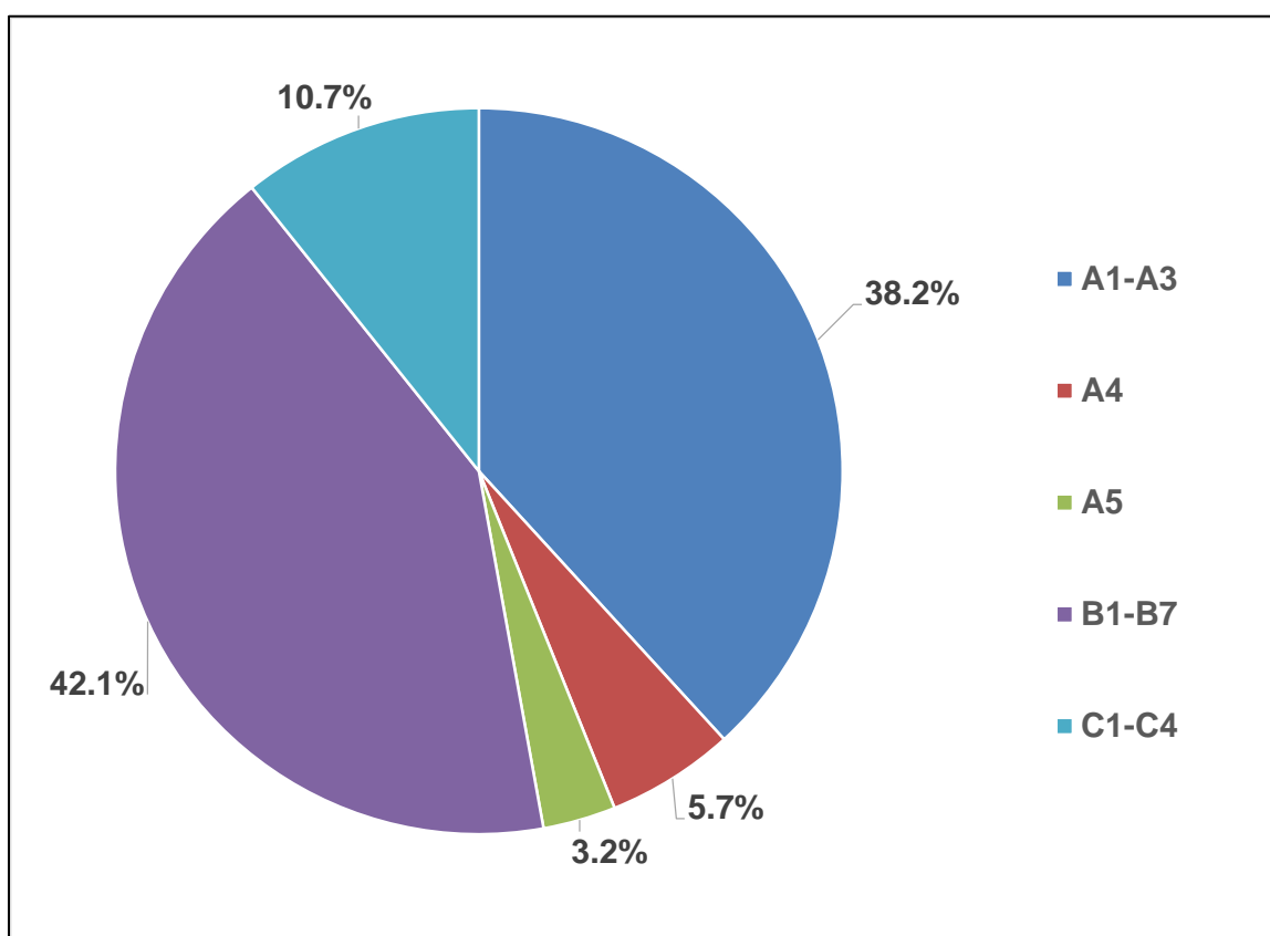
Figure 4: Process Dominance Analysis for the Production of 5/8 in. (15.9 mm) Securock® Brand UltraLight Coated and Uncoated Glass-Mat Roof Board
